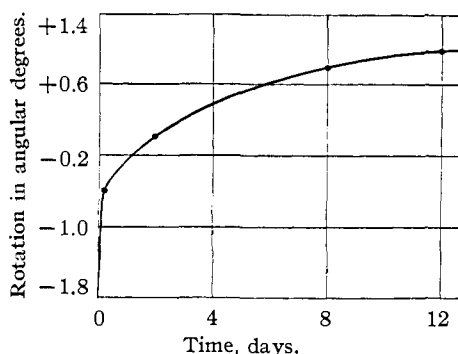
Fig. 2.—Mutarotation of 3-phenyl-4-hydroxycoumarin \beta -D-glucoside tetraacetate, 0.053 M in absolute methanol containing barium methoxide, 0.006 M .
